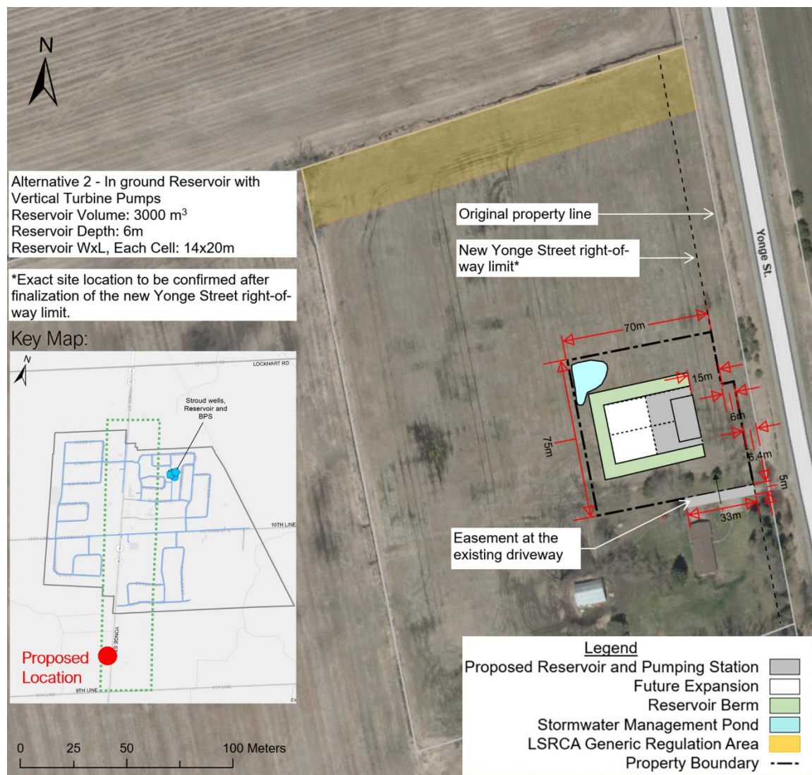
Figure 5.1 – Conceptual Site Layout of Preferred Alternative – At Location 2 with In-Ground Reservoir and Booster Pumping Station
